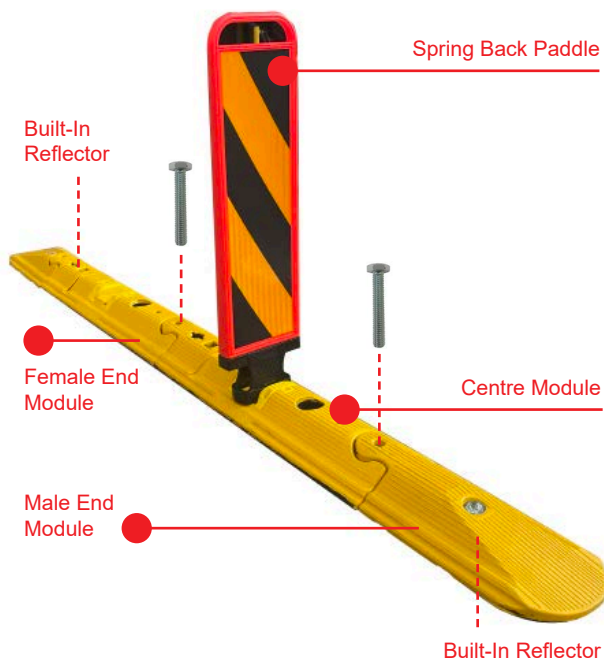
Assembled Traffic Lane Separator
