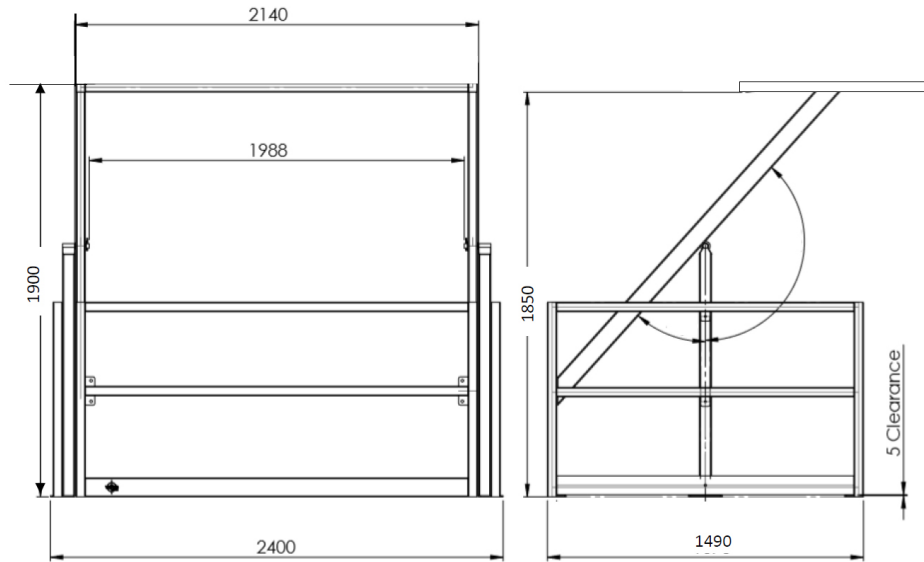
Low Profile Rollover Gate
