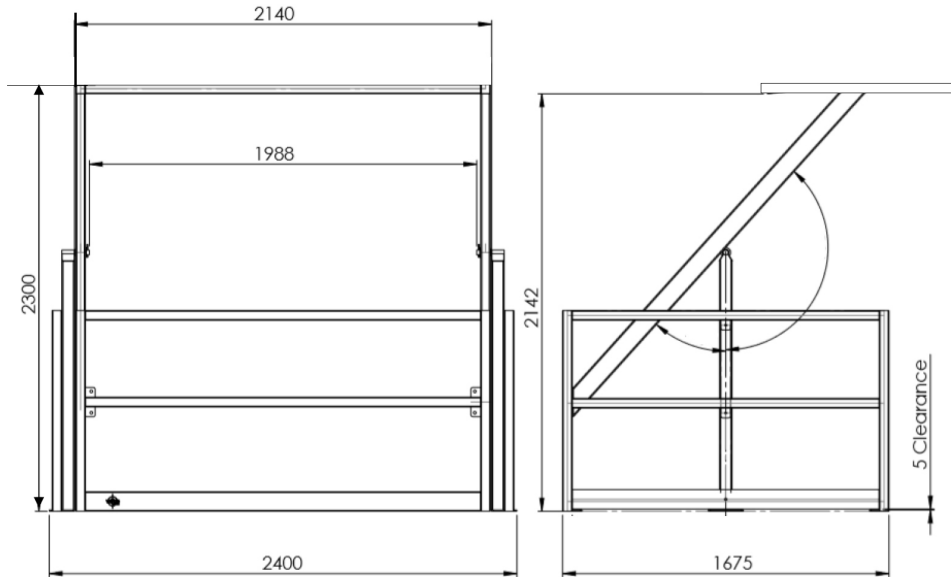
Standard Height Pallet Gate Overall Dimension: 2400mm W x 2300mm H To Suite Pallet: 1950mmW x 1250mm D x 1800mm H
